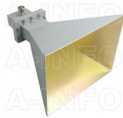
LB-340-15-C-7/16F Standard Gain Horn Antenna 2.2-3.3GHz 15dB Gain 7/16(DIN) Female
